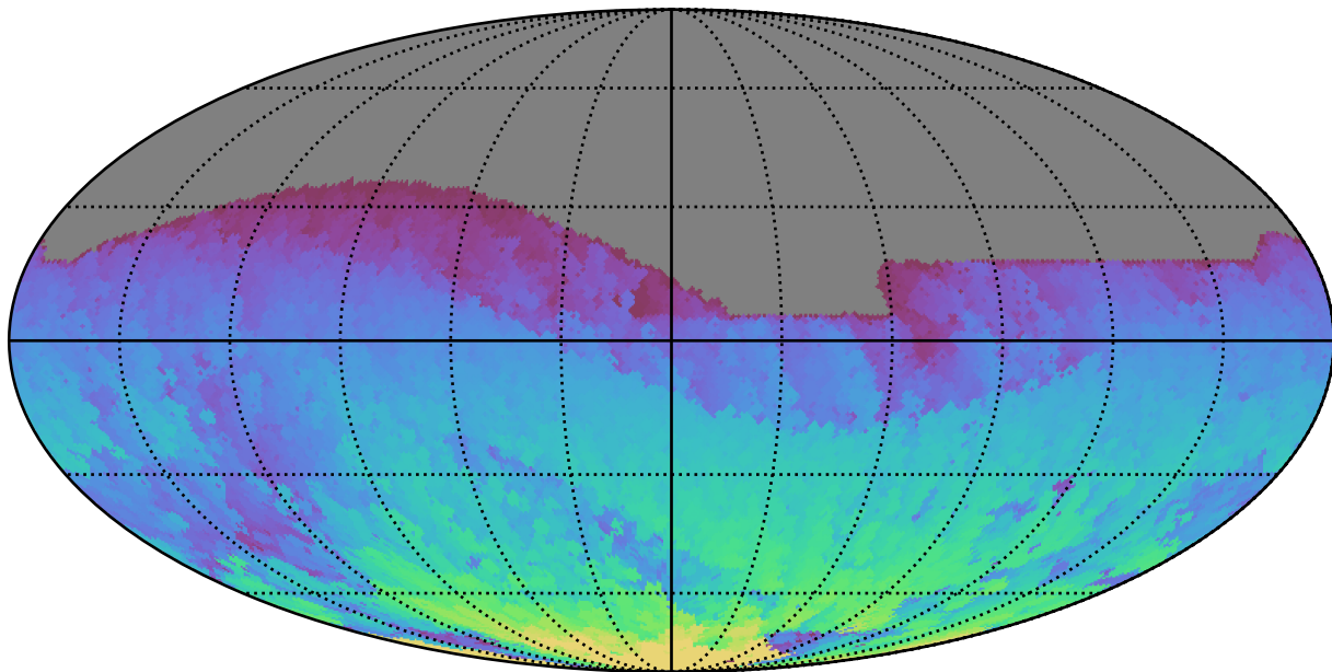
too_ignore_10_4v3.4_10yrs All sky z band: Max HA
