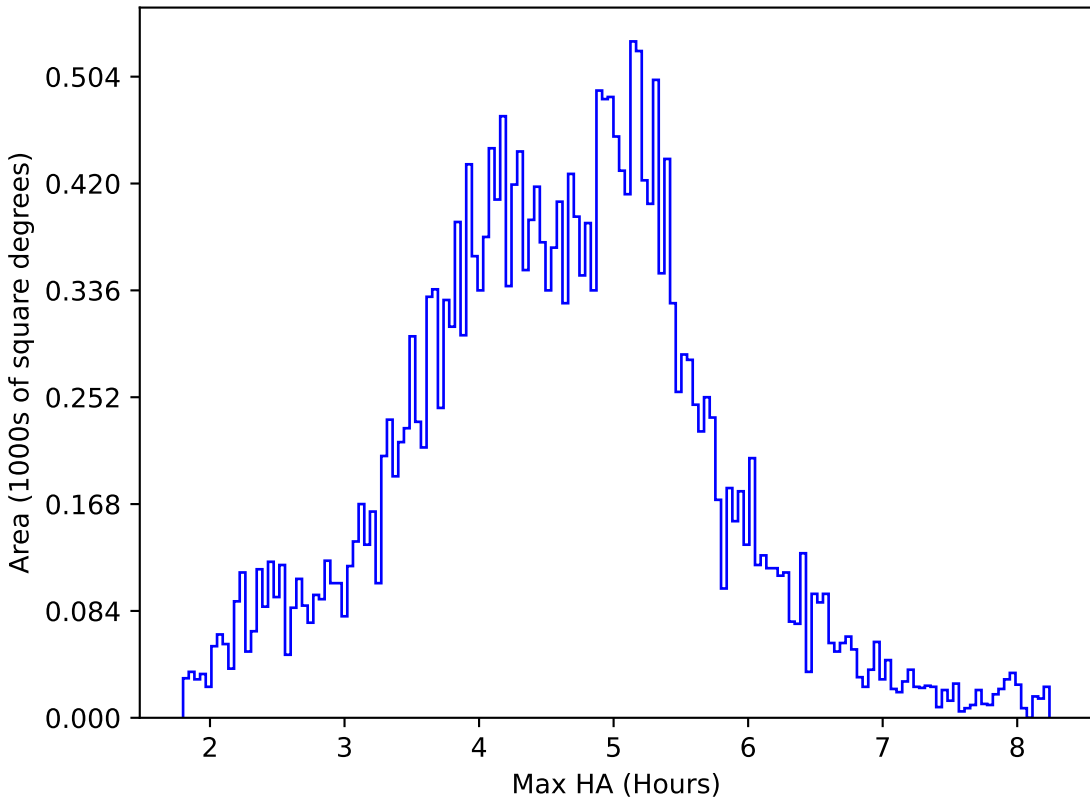
too_ignore_10_4v3.4_10yrs All sky z band: Max HA
