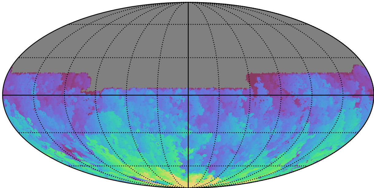
too_ignore_10_4v3.4_10yrs All sky u band: Max HA
