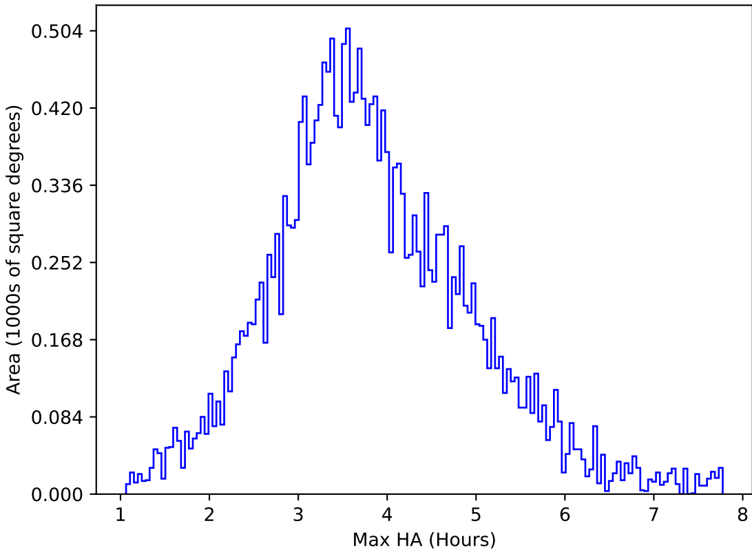
too_ignore_10_4v3.4_10yrs All sky u band: Max HA
