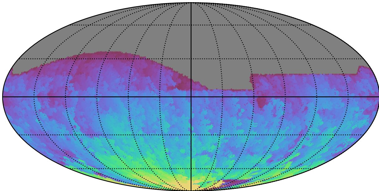
too_ignore_10_4v3.4_10yrs All sky r band: Max HA
