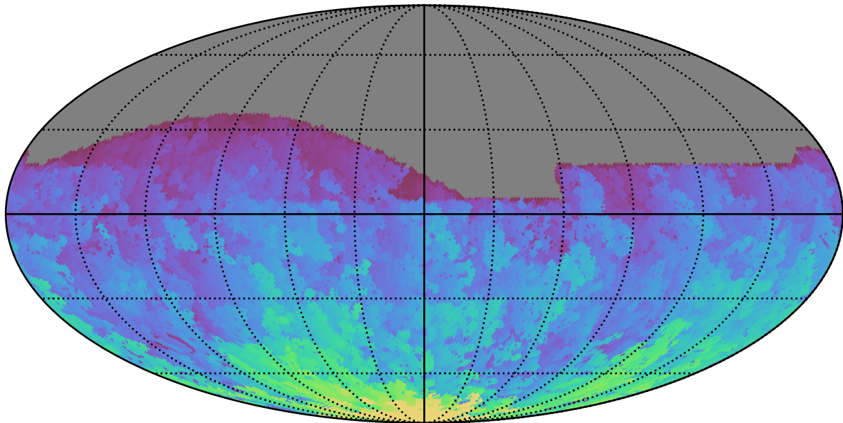
too_ignore_10_4v3.4_10yrs All sky g band: Max HA
