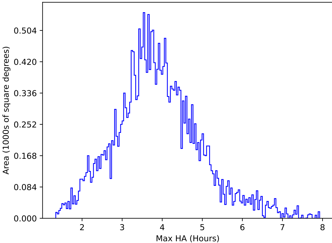
too_ignore_10_4v3.4_10yrs All sky g band: Max HA
