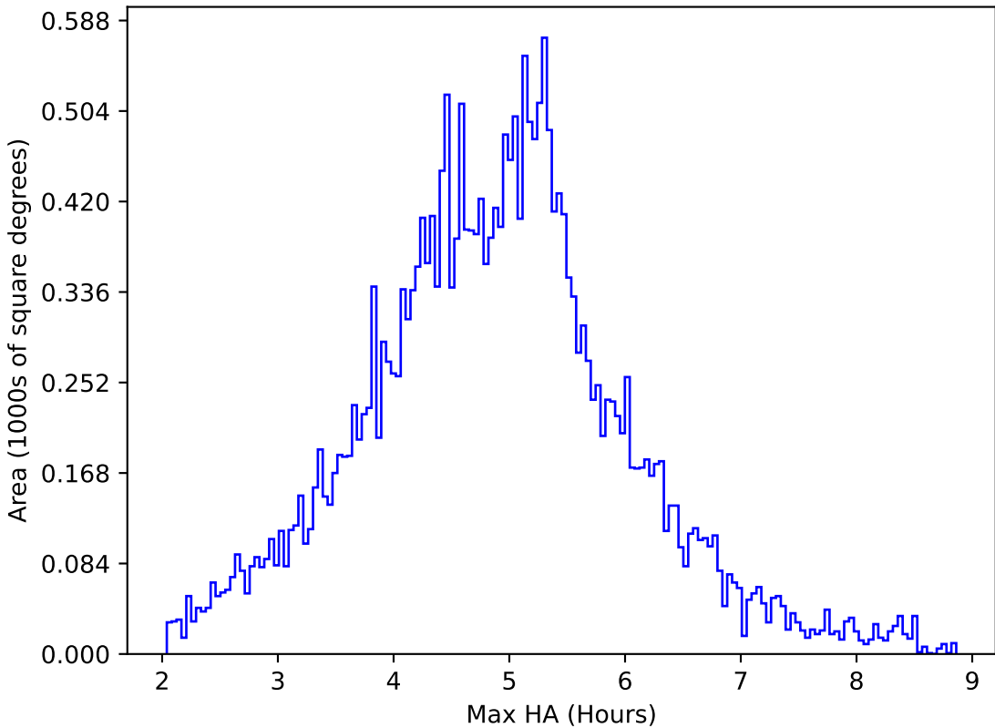
too_ignore_10_4v3.4_10yrs All sky all bands: Max HA
