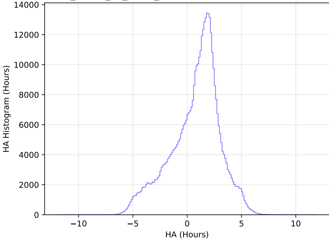
too_ignore_10_4v3.4_10yrs WFD z band: HA Histogram
