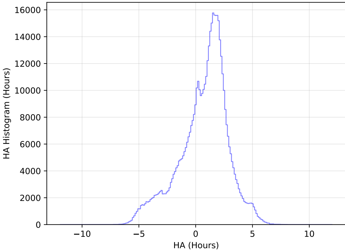
too_ignore_10_4v3.4_10yrs WFD i band: HA Histogram
