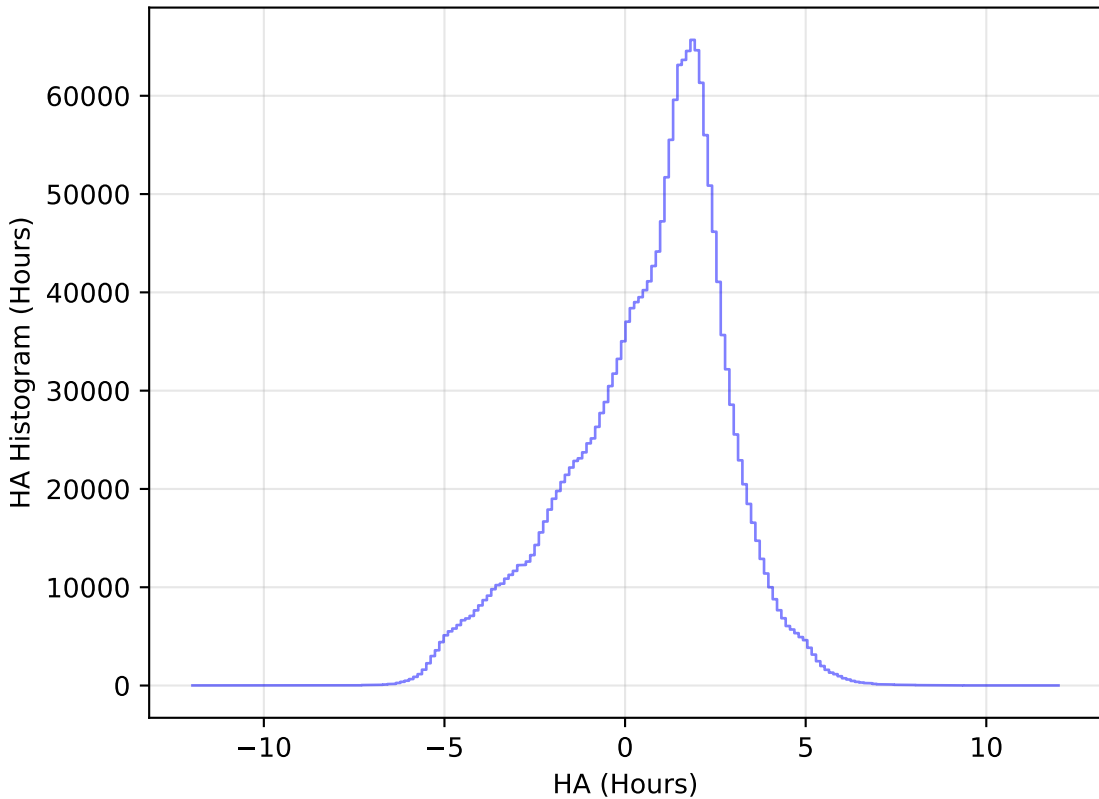
too_ignore_10_4v3.4_10yrs WFD all bands: HA Histogram
