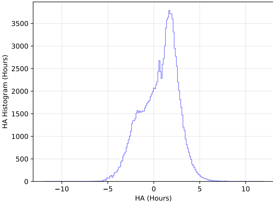
too_ignore_10_4v3.4_10yrs All sky u band: HA Histogram
