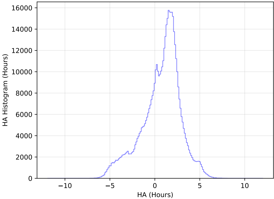
too_ignore_10_4v3.4_10yrs All sky i band: HA Histogram
