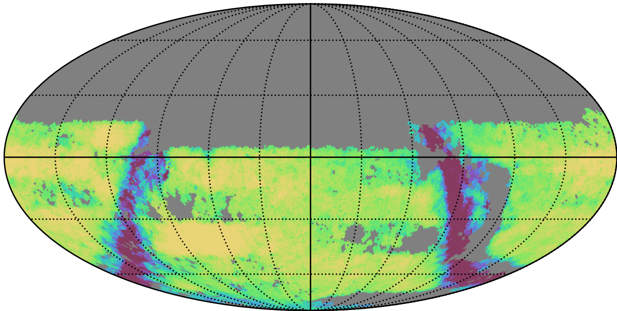
too_ignore_10_4v3.4_10yrs Yr 3-4 u band: Exgal_CoaddM5
