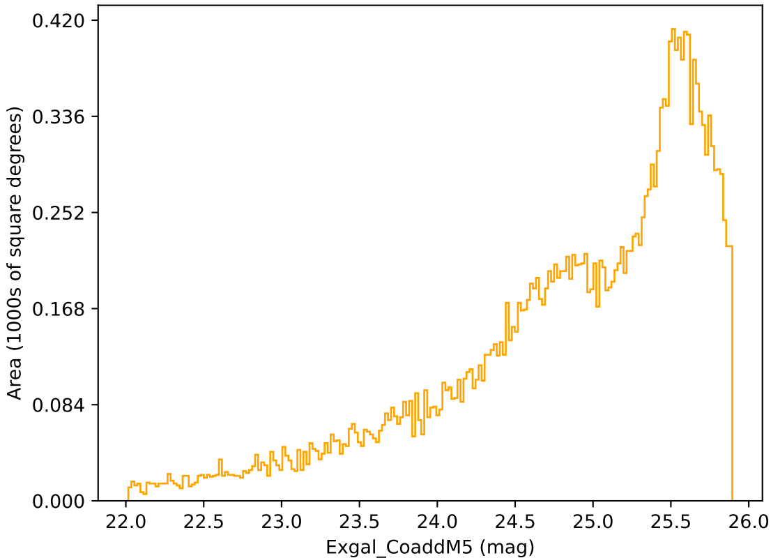
too_ignore_10_4v3.4_10yrs Yr 3-4 r band: Exgal_CoaddM5
