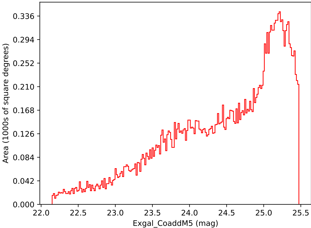
too_ignore_10_4v3.4_10yrs Yr 3-4 i band: Exgal_CoaddM5
