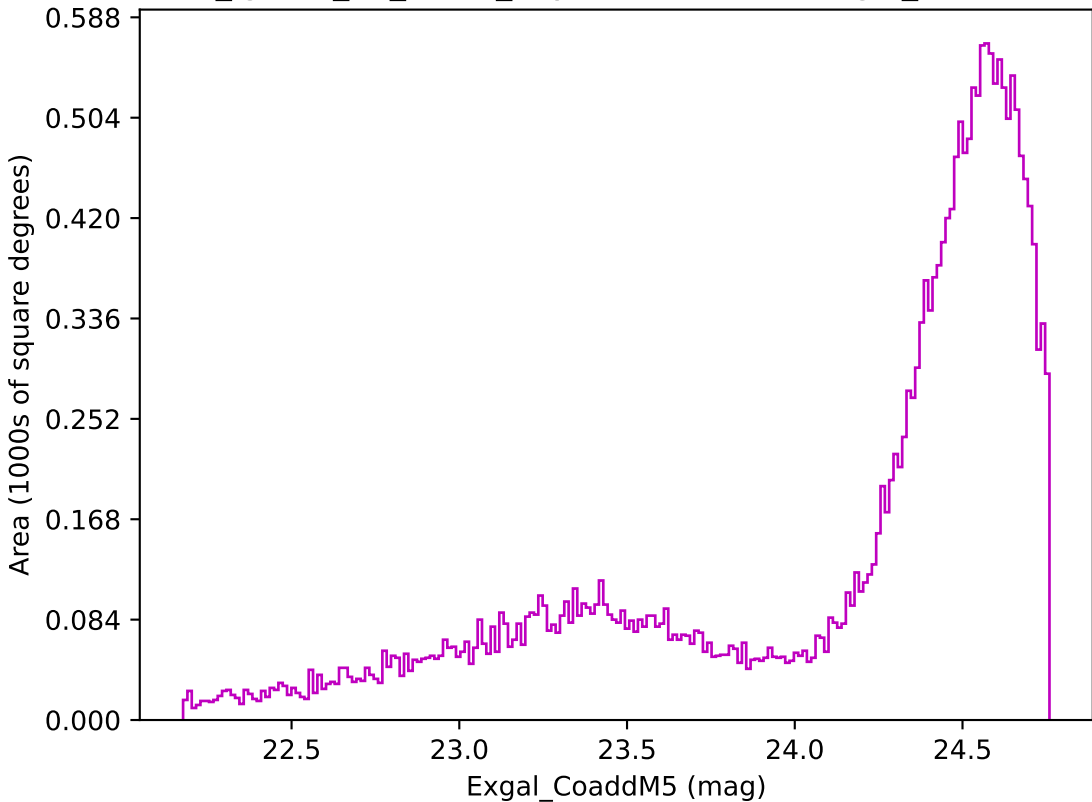
too_ignore_10_4v3.4_10yrs Yr 1 z band: Exgal_CoaddM5
