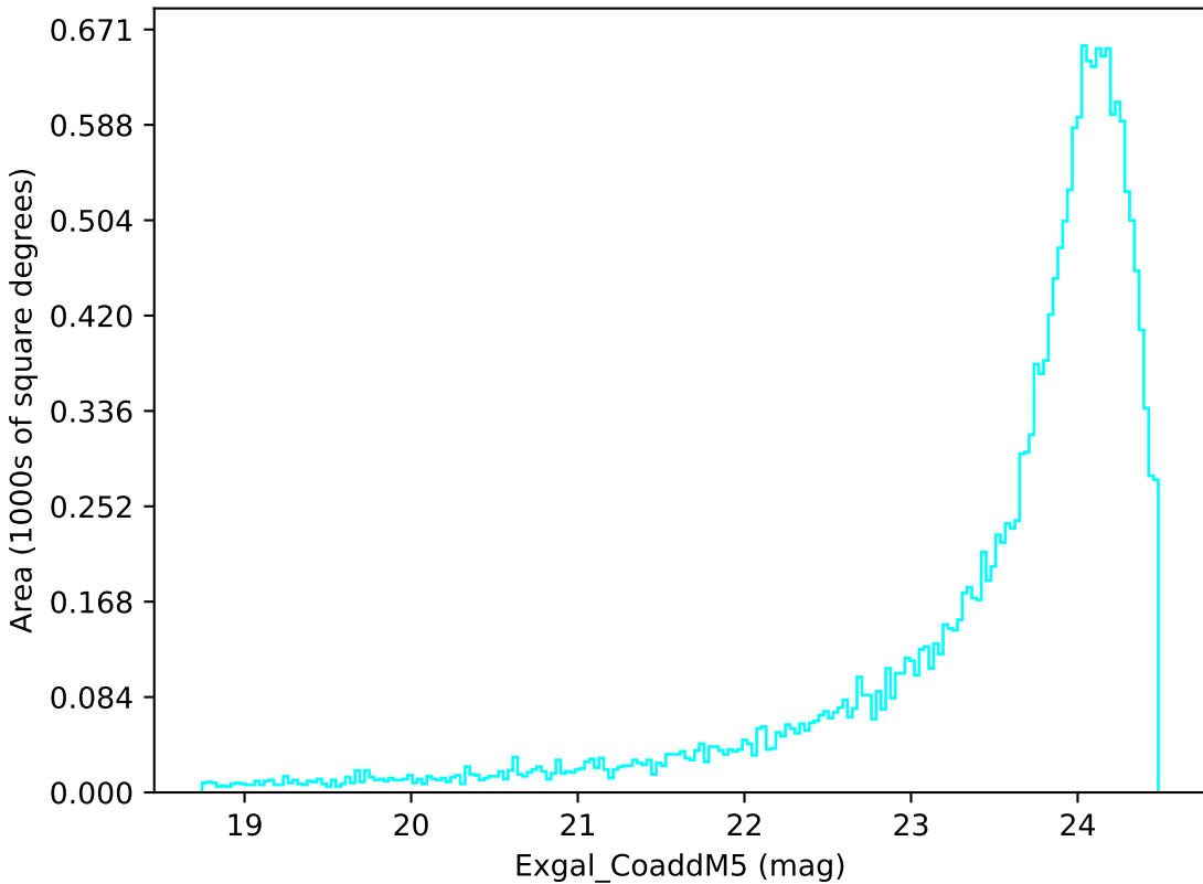
too_ignore_10_4v3.4_10yrs Yr 1 u band: Exgal_CoaddM5
