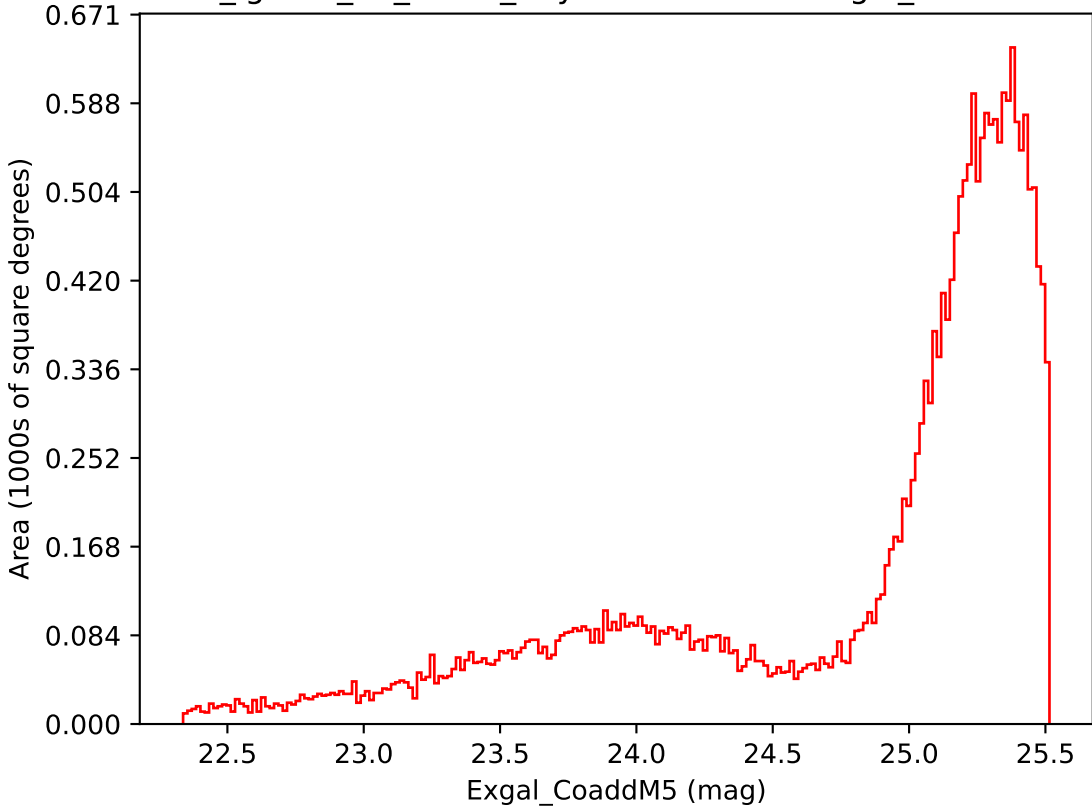
too_ignore_10_4v3.4_10yrs Yr 1 i band: Exgal_CoaddM5
