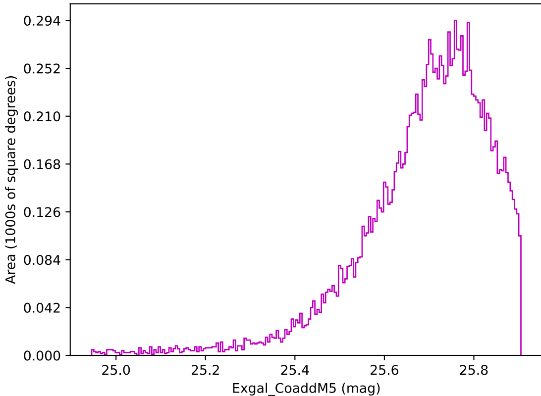
too_ignore_10_4v3.4_10yrs WFD z band: Exgal_CoaddM5
