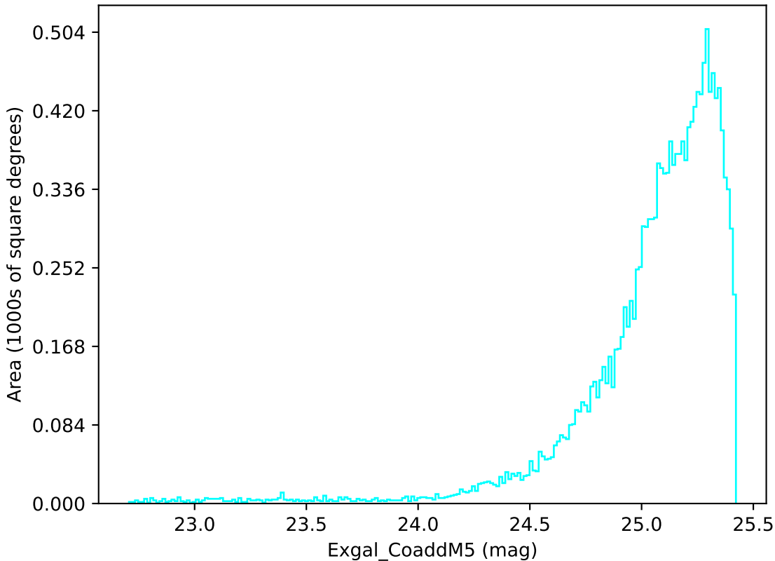
too_ignore_10_4v3.4_10yrs WFD u band: Exgal_CoaddM5
