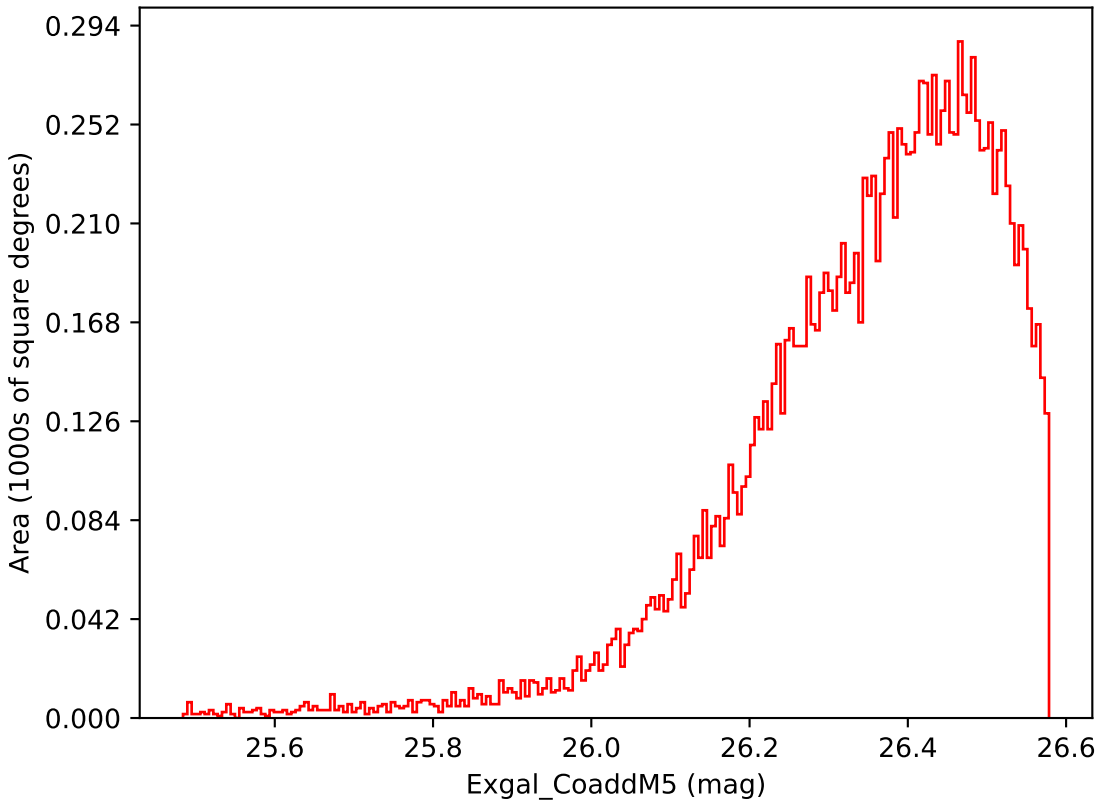
too_ignore_10_4v3.4_10yrs WFD i band: Exgal_CoaddM5
