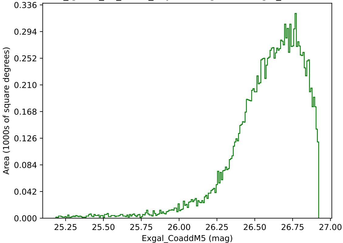
too_ignore_10_4v3.4_10yrs WFD g band: Exgal_CoaddM5
