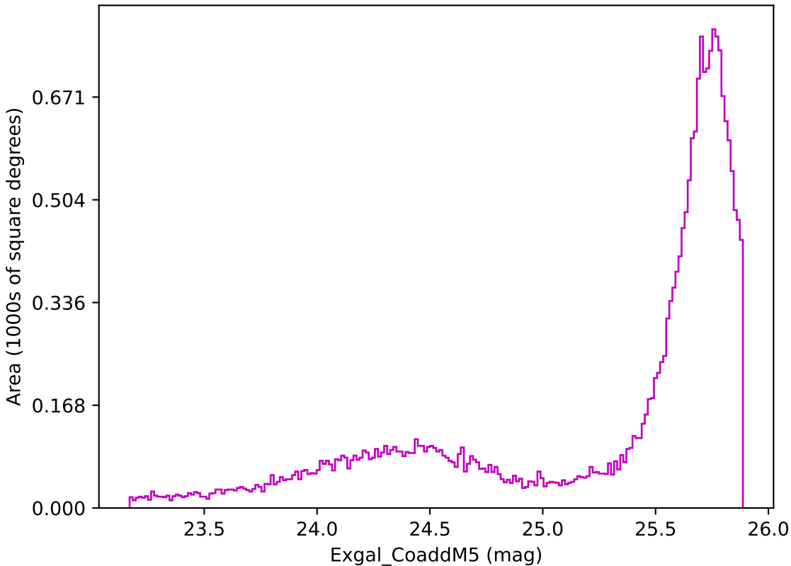
too_ignore_10_4v3.4_10yrs All sky z band: Exgal_CoaddM5
