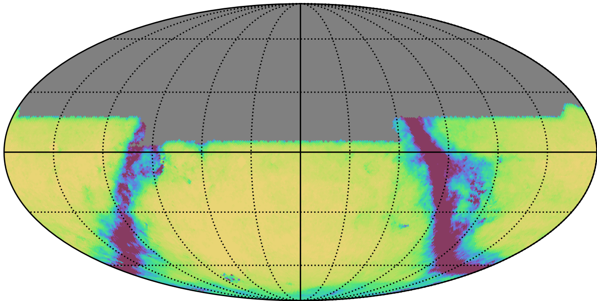
too_ignore_10_4v3.4_10yrs All sky u band: Exgal_CoaddM5
