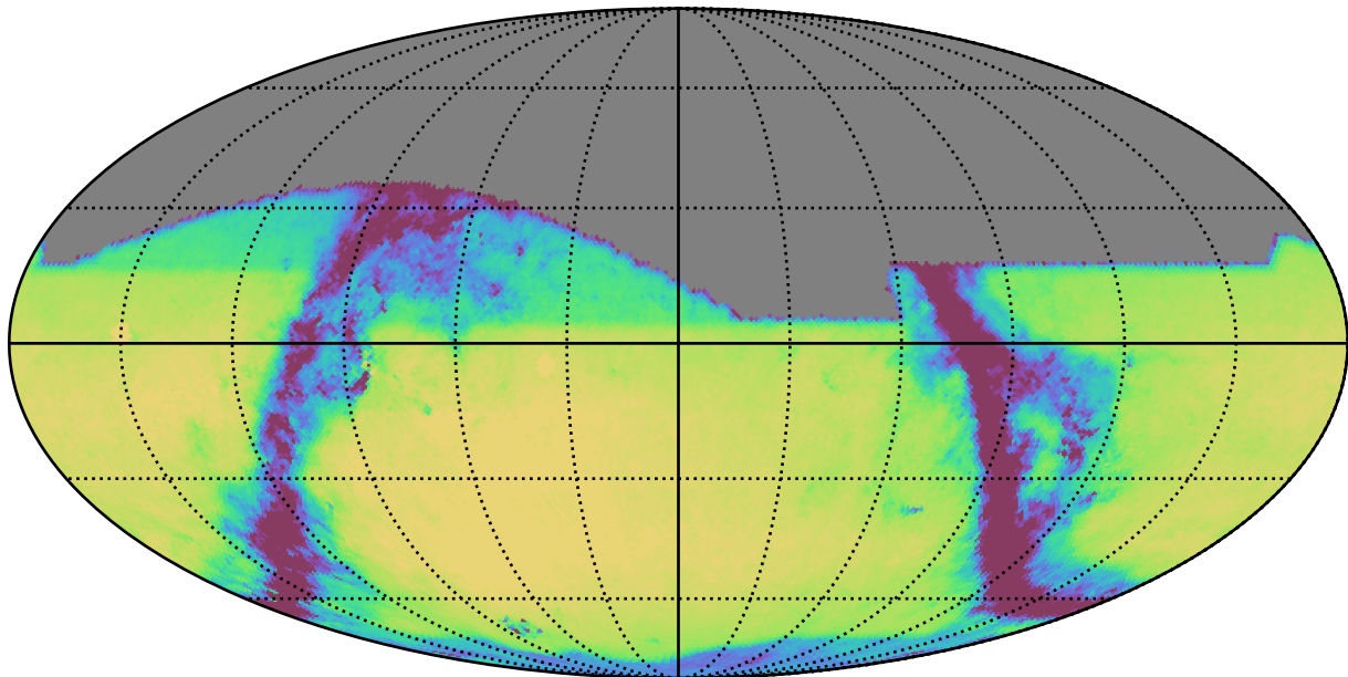
too_ignore_10_4v3.4_10yrs All sky r band: Exgal_CoaddM5
