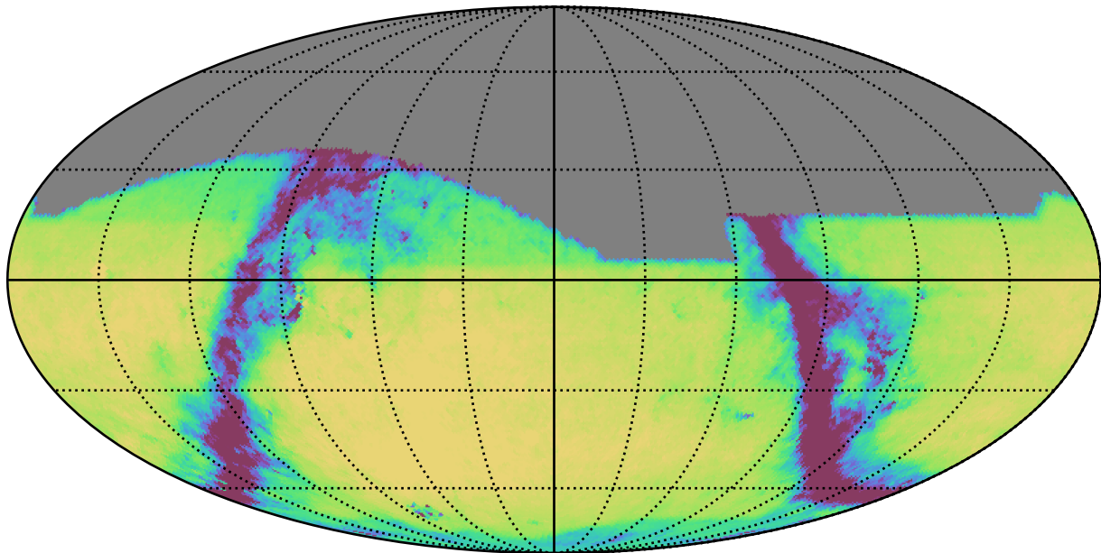
too_ignore_10_4v3.4_10yrs All sky g band: Exgal_CoaddM5
