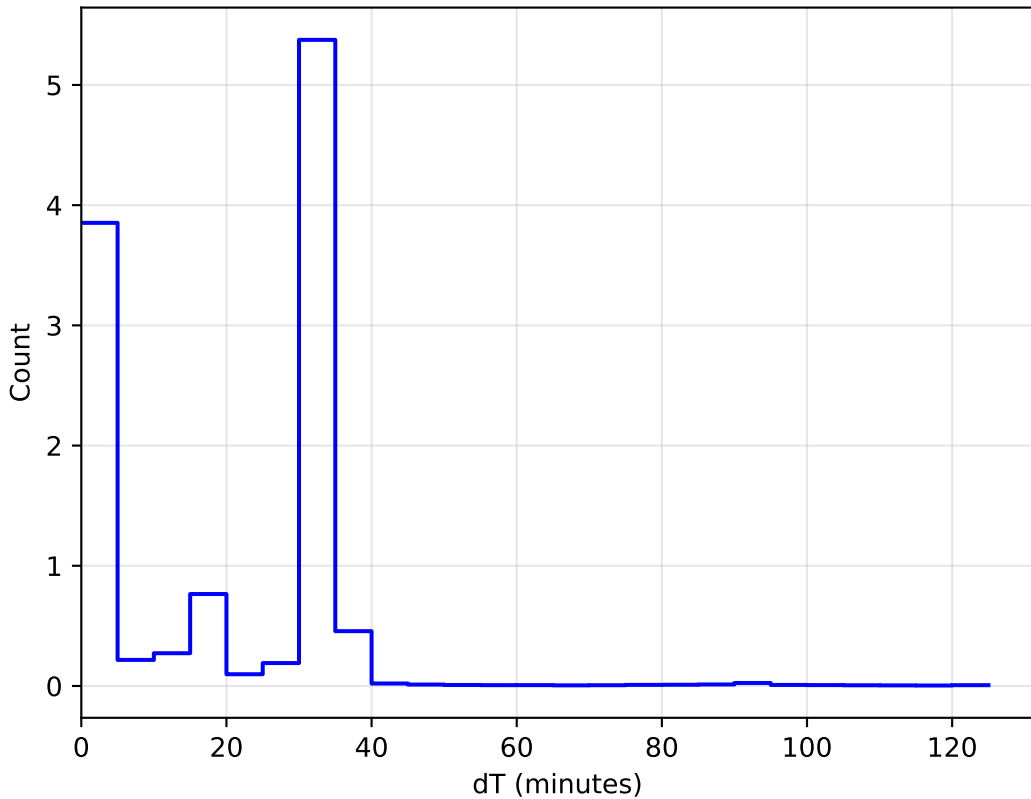
1e6 too_ignore_10_4v3.4_10yrs WFD: DeltaT Histogram
