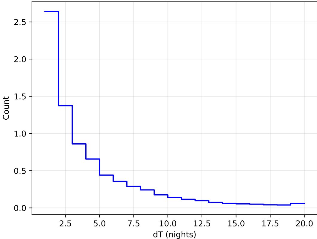
too_ignore_10_4v3.4_10yrs WFD all bands: DeltaNight Histogram 1e6
