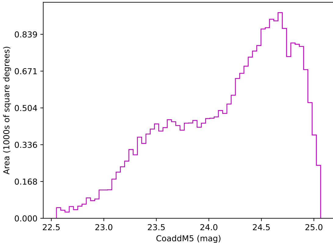
too_ignore_10_4v3.4_10yrs Yr 3-4 z band: CoaddM5
