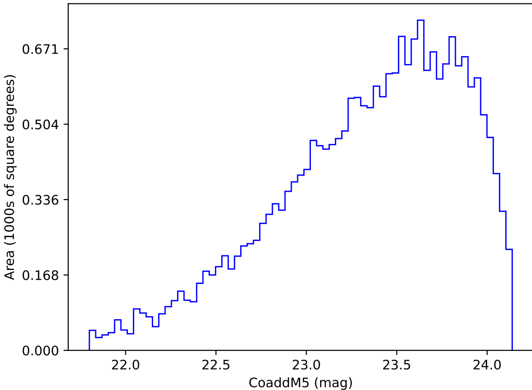
too_ignore_10_4v3.4_10yrs Yr 3-4 y band: CoaddM5
