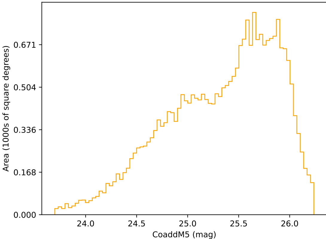
too_ignore_10_4v3.4_10yrs Yr 3-4 r band: CoaddM5
