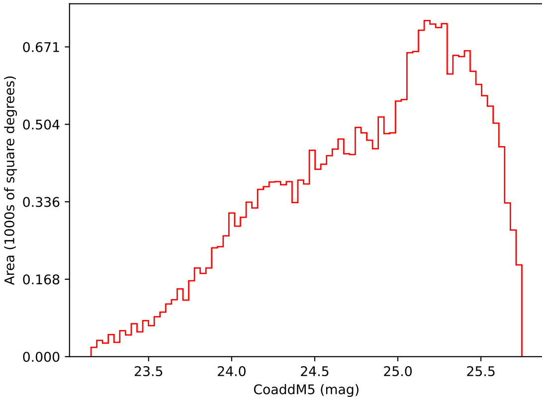
too_ignore_10_4v3.4_10yrs Yr 3-4 i band: CoaddM5
