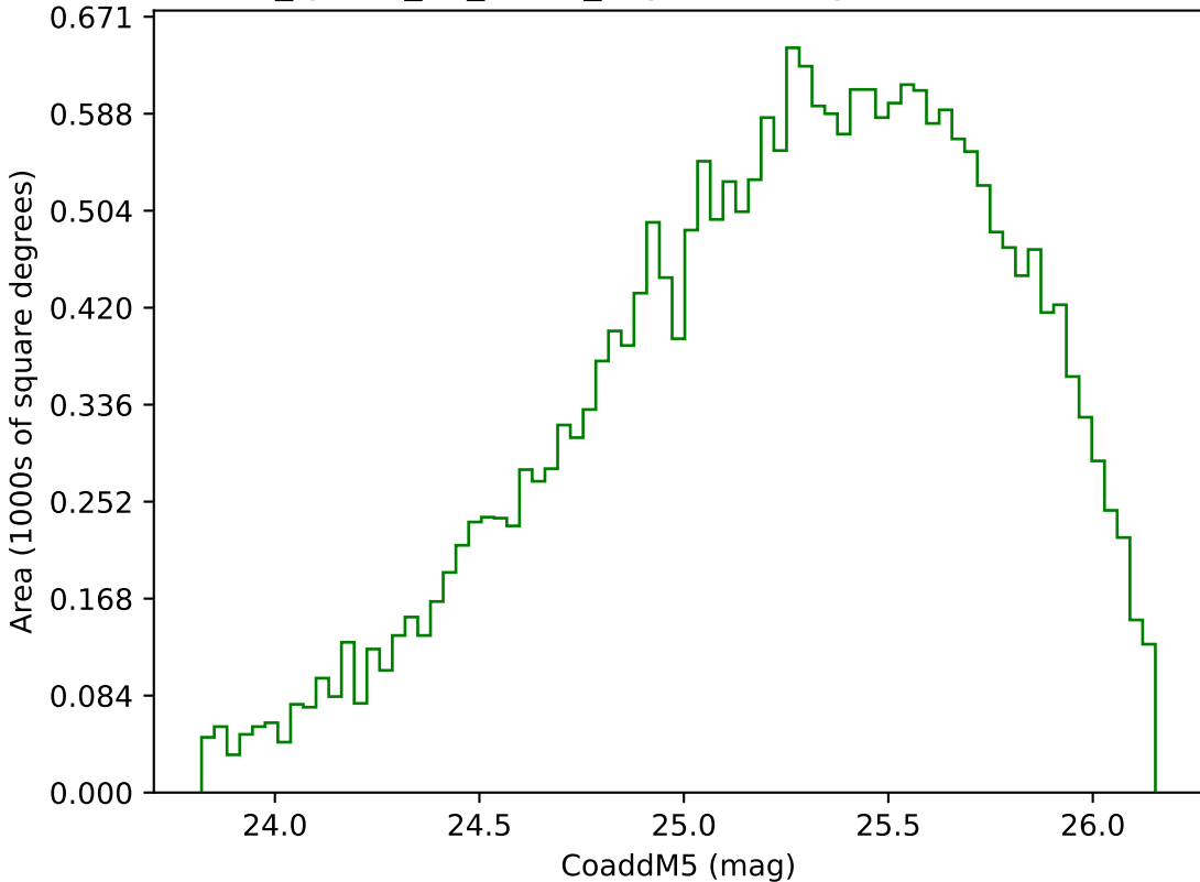
too_ignore_10_4v3.4_10yrs Yr 3-4 g band: CoaddM5
