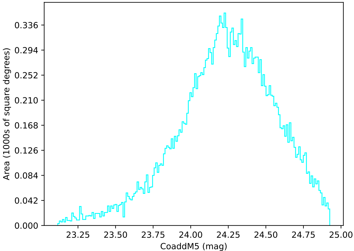
too_ignore_10_4v3.4_10yrs Yr 1 u band: CoaddM5
