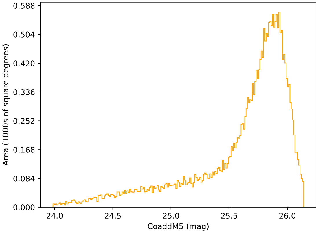
too_ignore_10_4v3.4_10yrs Yr 1 r band: CoaddM5
