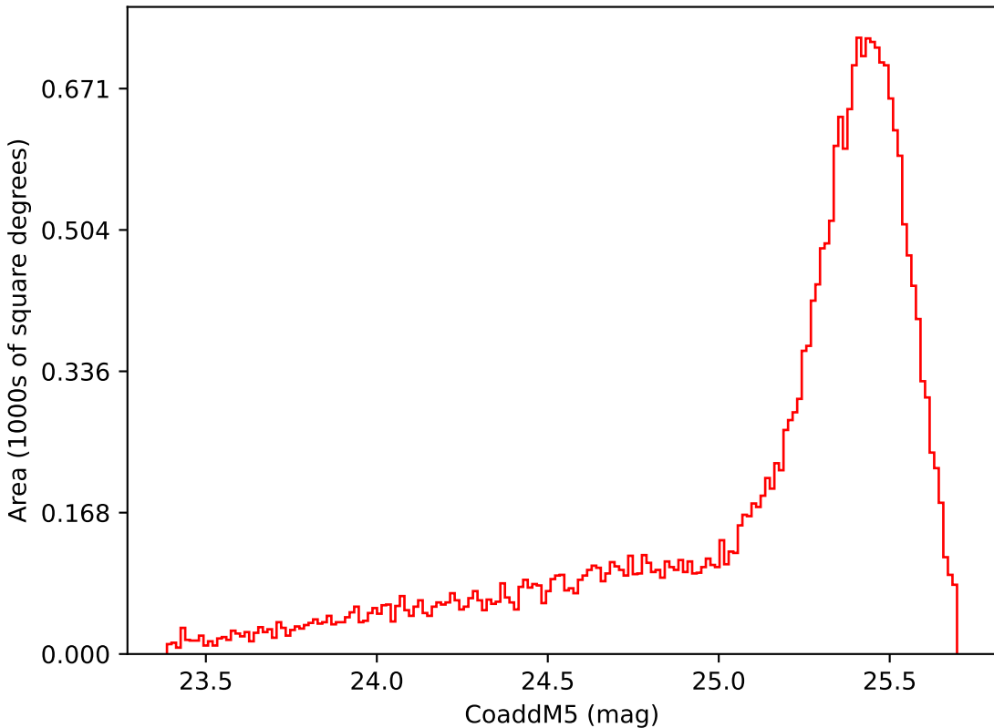
too_ignore_10_4v3.4_10yrs Yr 1 i band: CoaddM5
