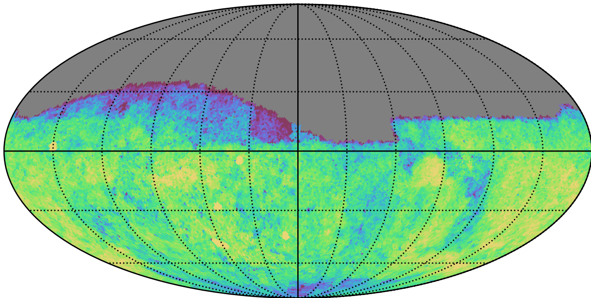
too_ignore_10_4v3.4_10yrs Yr 1 g band: CoaddM5
