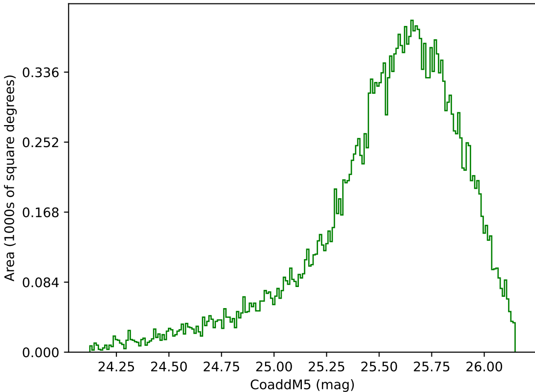
too_ignore_10_4v3.4_10yrs Yr 1 g band: CoaddM5
