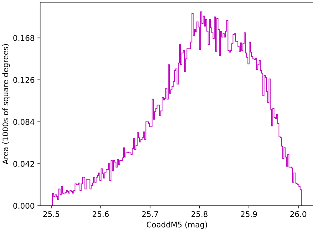
too_ignore_10_4v3.4_10yrs WFD z band: CoaddM5
