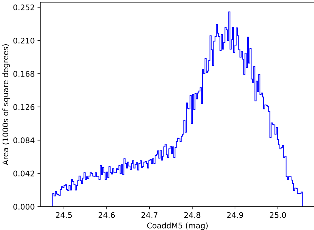
too_ignore_10_4v3.4_10yrs WFD y band: CoaddM5
