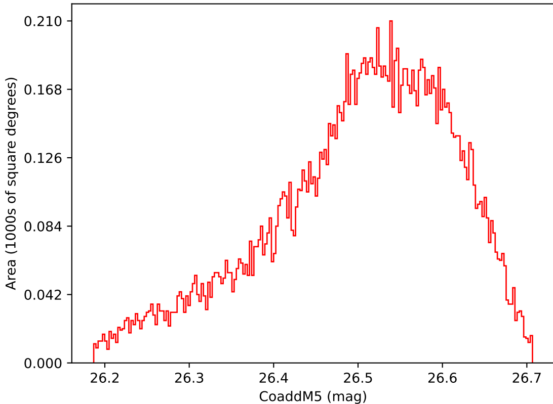
too_ignore_10_4v3.4_10yrs WFD i band: CoaddM5
