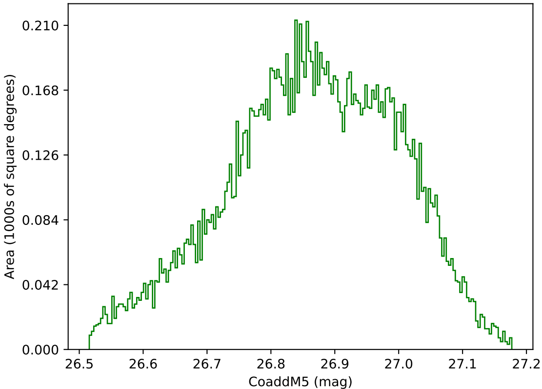
too_ignore_10_4v3.4_10yrs WFD g band: CoaddM5
