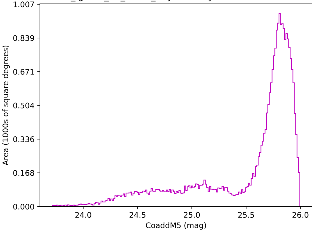
too_ignore_10_4v3.4_10yrs All sky z band: CoaddM5
