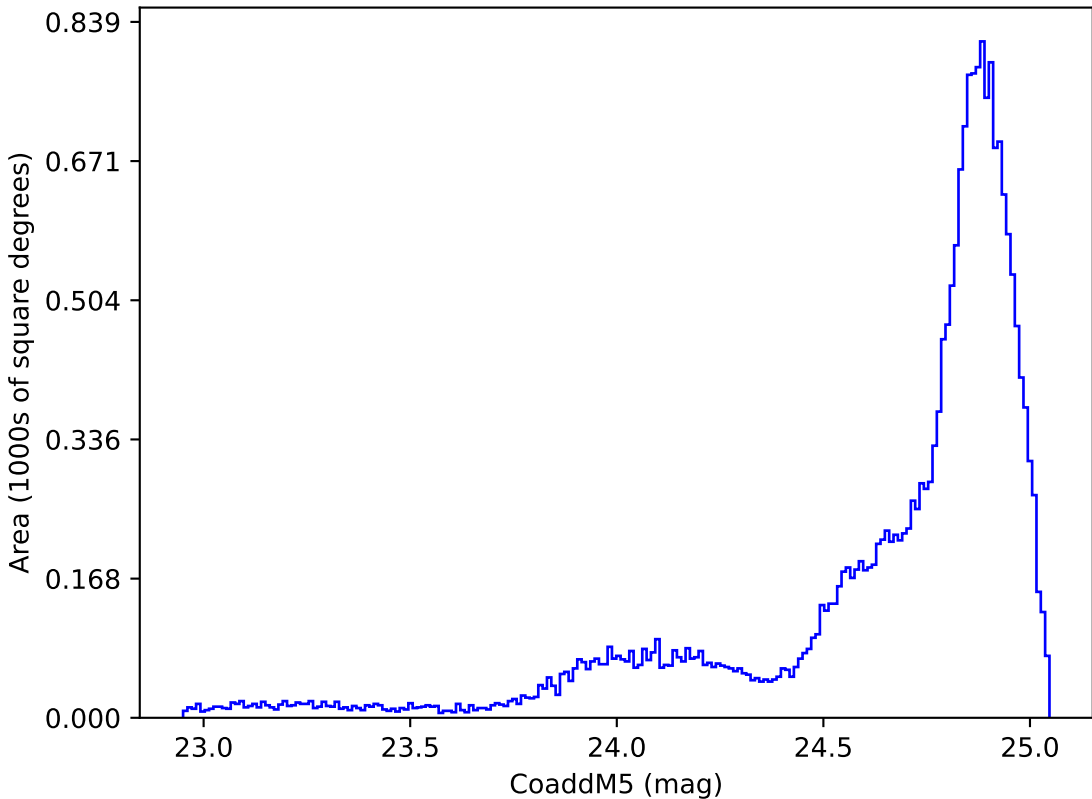
too_ignore_10_4v3.4_10yrs All sky y band: CoaddM5
