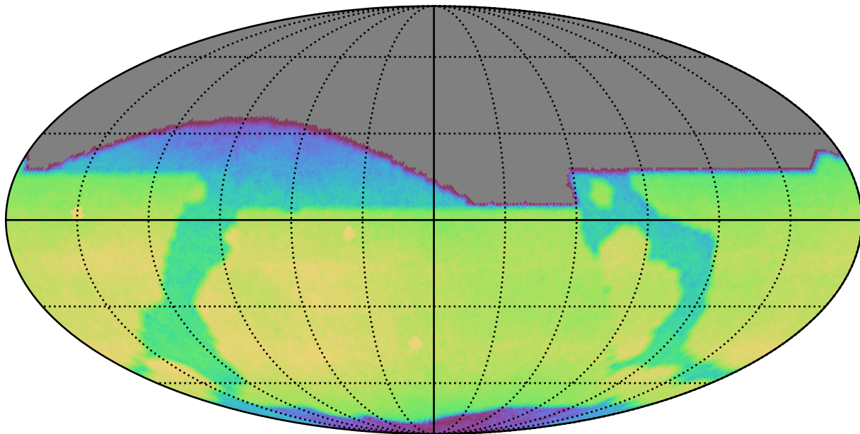
too_ignore_10_4v3.4_10yrs All sky r band: CoaddM5
