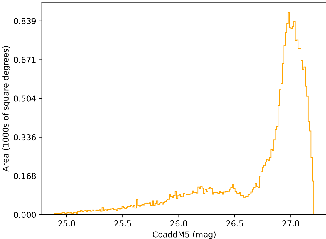
too_ignore_10_4v3.4_10yrs All sky r band: CoaddM5
