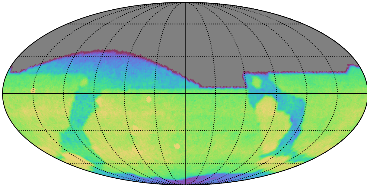
too_ignore_10_4v3.4_10yrs All sky g band: CoaddM5
