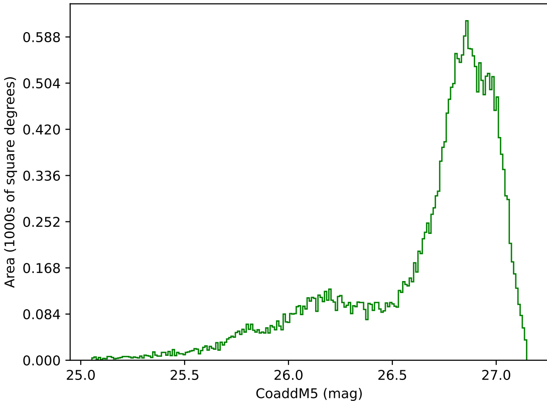
too_ignore_10_4v3.4_10yrs All sky g band: CoaddM5
