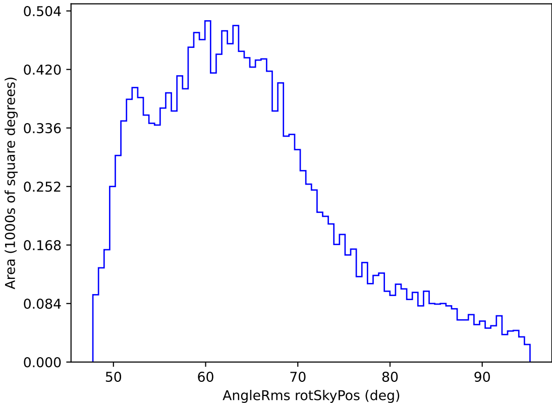
too_ignore_10_4v3.4_10yrs WFD z band: AngleRms rotSkyPos
